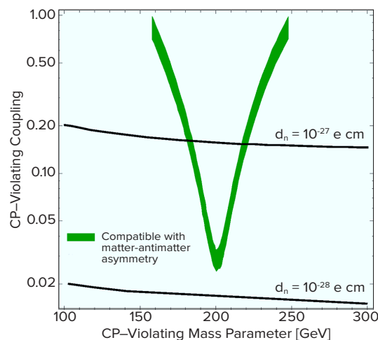
Figure 5.5: The relationship between the relevant parameters in the minimal Supersymmetric Standard Model that are needed to account for the observed excess of matter over antimatter is shown as the green band. The nearly horizontal lines indicate the size of a neutron EDM as a function of these parameters. The neutron EDM search being developed at the FNPB would probe nearly all of this parameter space.
